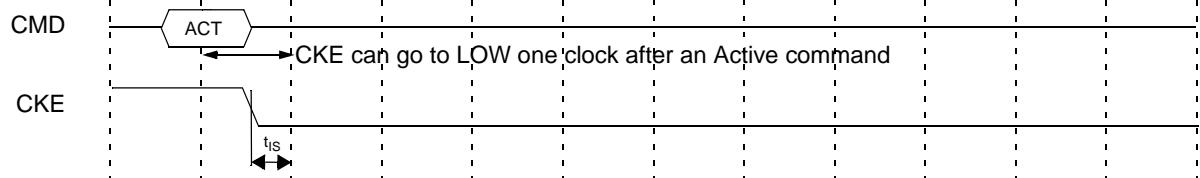
Figure 52. Active command to power down entry
