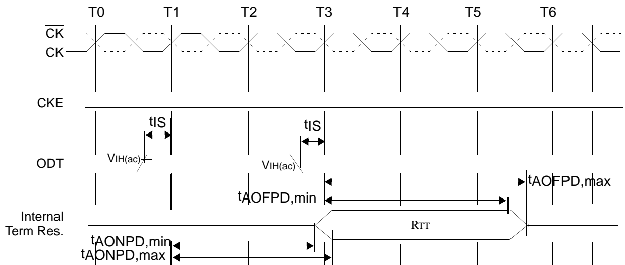
Figure 12. ODT timing for powerdown mode
