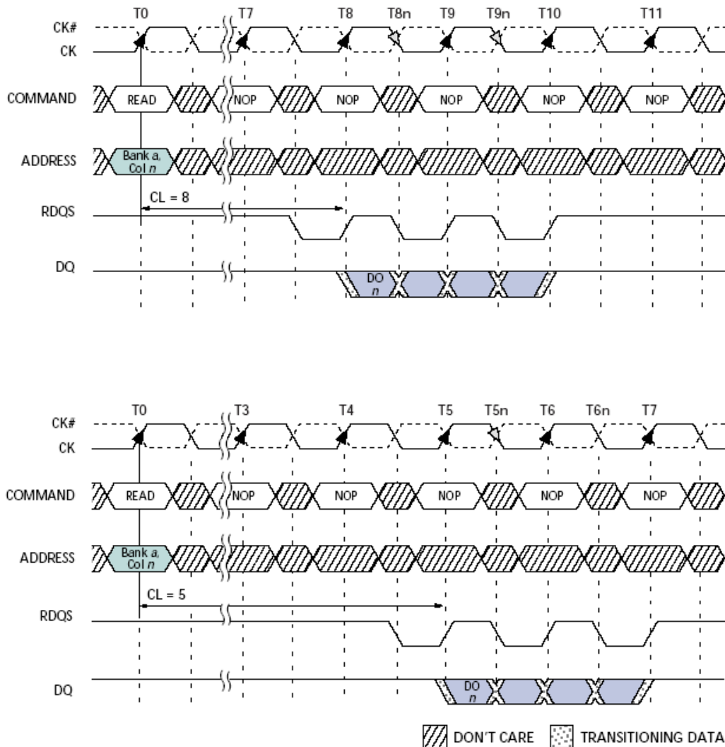
Figure 12: READ Burst
