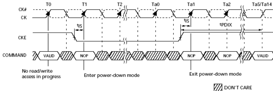
Figure 26: Power-Down
