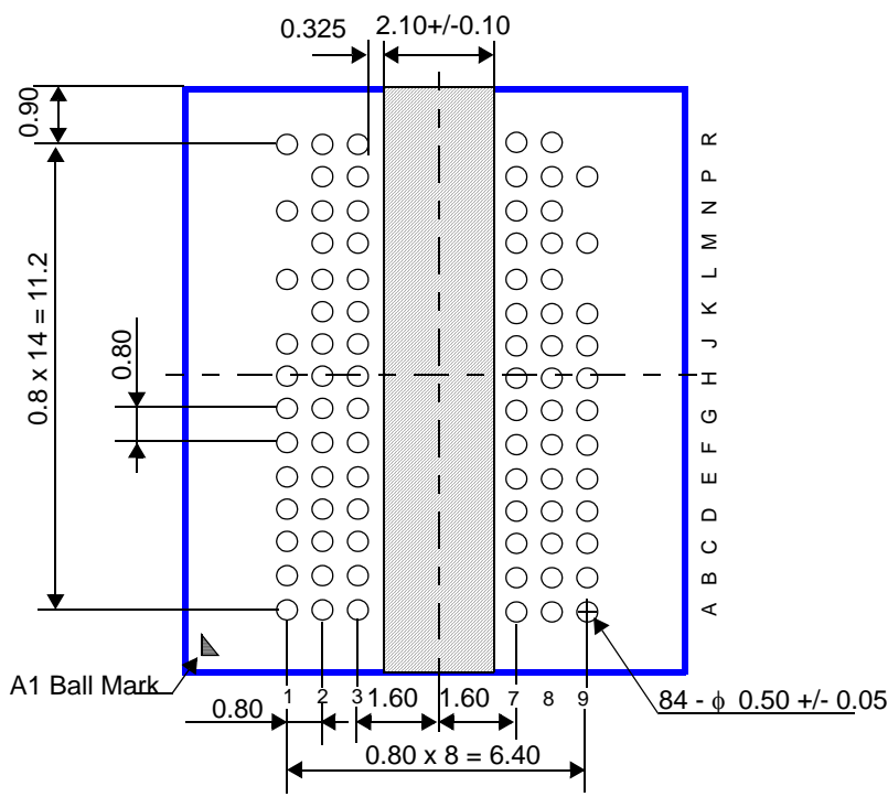
<Bottom View>
